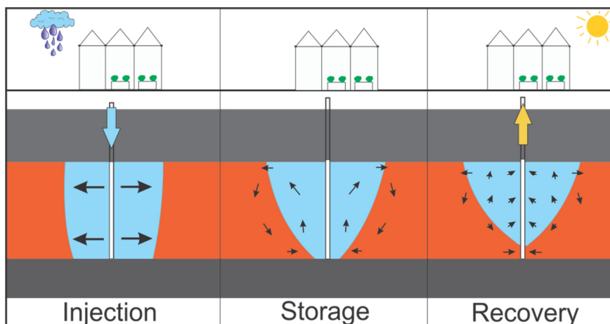
Figure 2: Freshwater loss during ASR in brackish and saltwater aquifers due to buoyancy effects.
