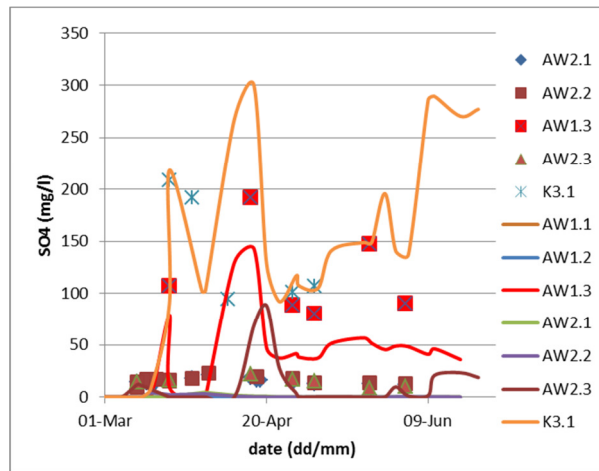
Figure 11: Modelled and observed \text{SO}_4 -concentrations at the most relevant well screens.
