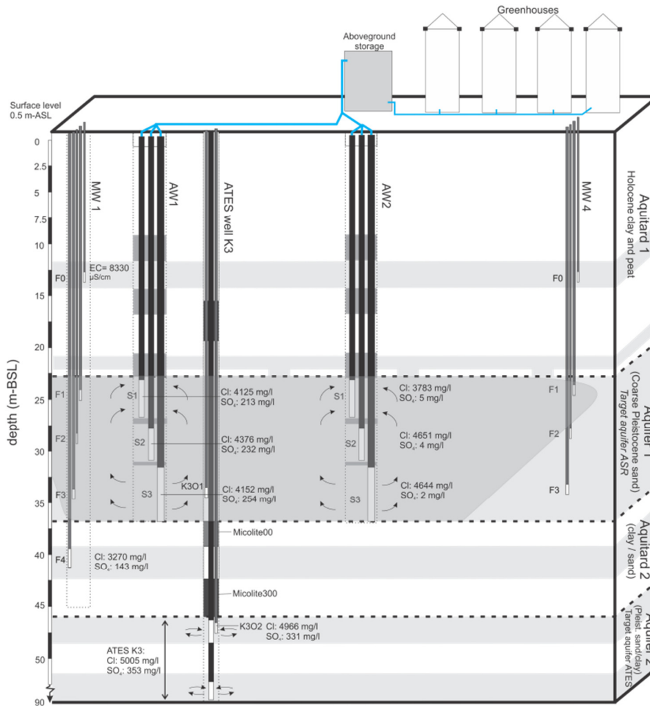
Figure 5: Cross-section of the Westland ASR-pilot, including the ambient groundwater quality observed preceding the ASR operation.
