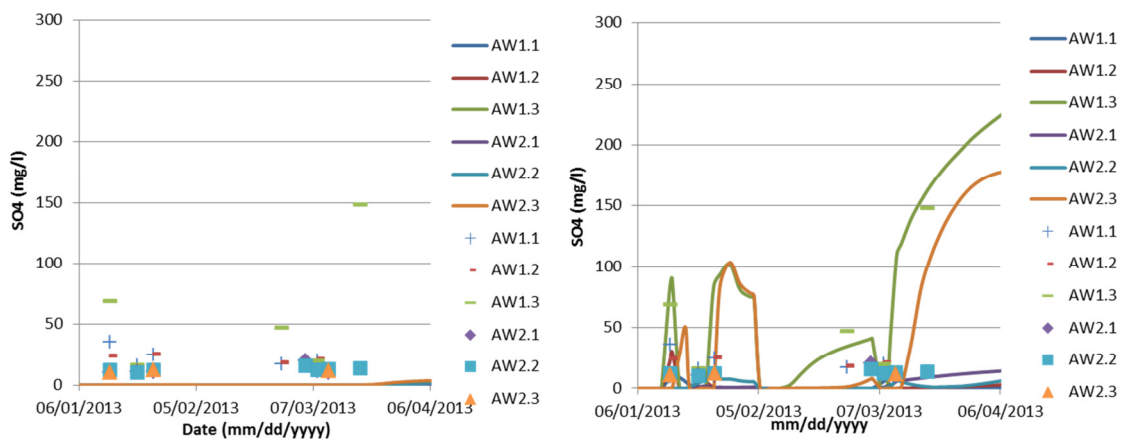
Figure 9: Modelled (solid lines) and observed (data points) SO_4 -concentrations. High concentrations indicate admixing of deeper saltwater. Left = no borehole leakage, right = borehole leakage via a 1x1 m borehole with K=1000 m/d).
