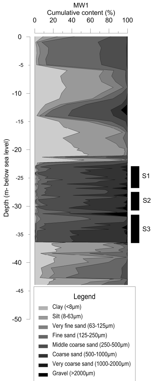
Figure 6: Cumulative grain size contents observed at MW1 (at 5 m from ASR well 1). S1-S3 mark the depth intervals of the ASR well screens.
