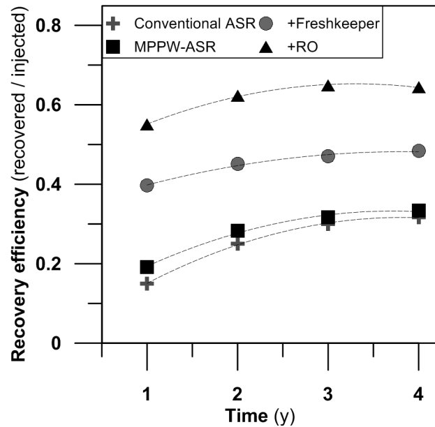
Figure 14: Recovery efficiencies at the Westland ASR site without the borehole leakage resulting from the SEAWAT groundwater transport model for a conventional ASR well (one well screen, fully penetrating), multiple partially penetrating wells without a ‘Freshkeeper’ (scenario MPPW-ASR), for a MPPW in combination with a ‘Freshkeeper’ (scenario +Freshkeeper), and for a scenario in which RO is applied on the intercepted brackish water to produce additional freshwater (50% of the flux).
