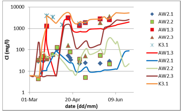
Figure 12: Modelled and observed Cl-concentrations at the most relevant well screens.
