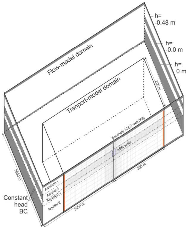
Figure 7: Set-up of the Westland ASR groundwater transport model (half-domain).
