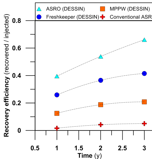
Figure 15: Recovery efficiencies at the Westland ASR site assuming a doubled target aquifer thickness resulting from the SEAWAT groundwater transport model for a conventional ASR well (one well screen, fully penetrating), multiple partially penetrating wells without a 'Freshkeeper' (scenario MPPW), for a MPPW in combination with a 'Freshkeeper' (scenario Freshkeeper), and for a scenario in which RO is applied on the intercepted brackish water to produce additional freshwater (50% of the flux).
