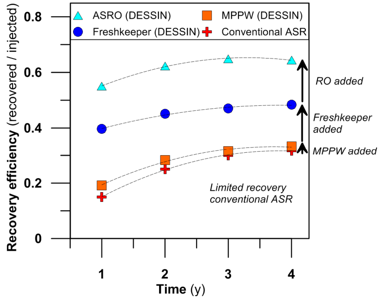
Figure 16: Most relevant results of the SEAWAT modelling study: an increase in recovery efficiencies at the Westland target aquifer thanks to the introduction of the MPPW, the Freshkeeper, and ASRO.
