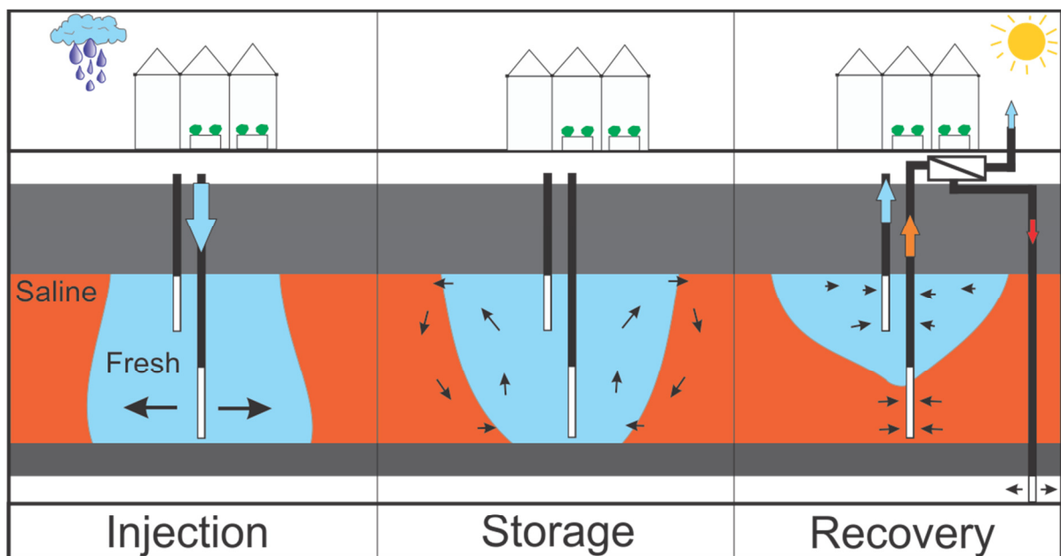
Figure 3: The introduction of the MPPW for deep injection and shallow recovery in combination with a Freshkeeper and optional RO-treatment for a maximal recovery of freshwater (ASRO).
