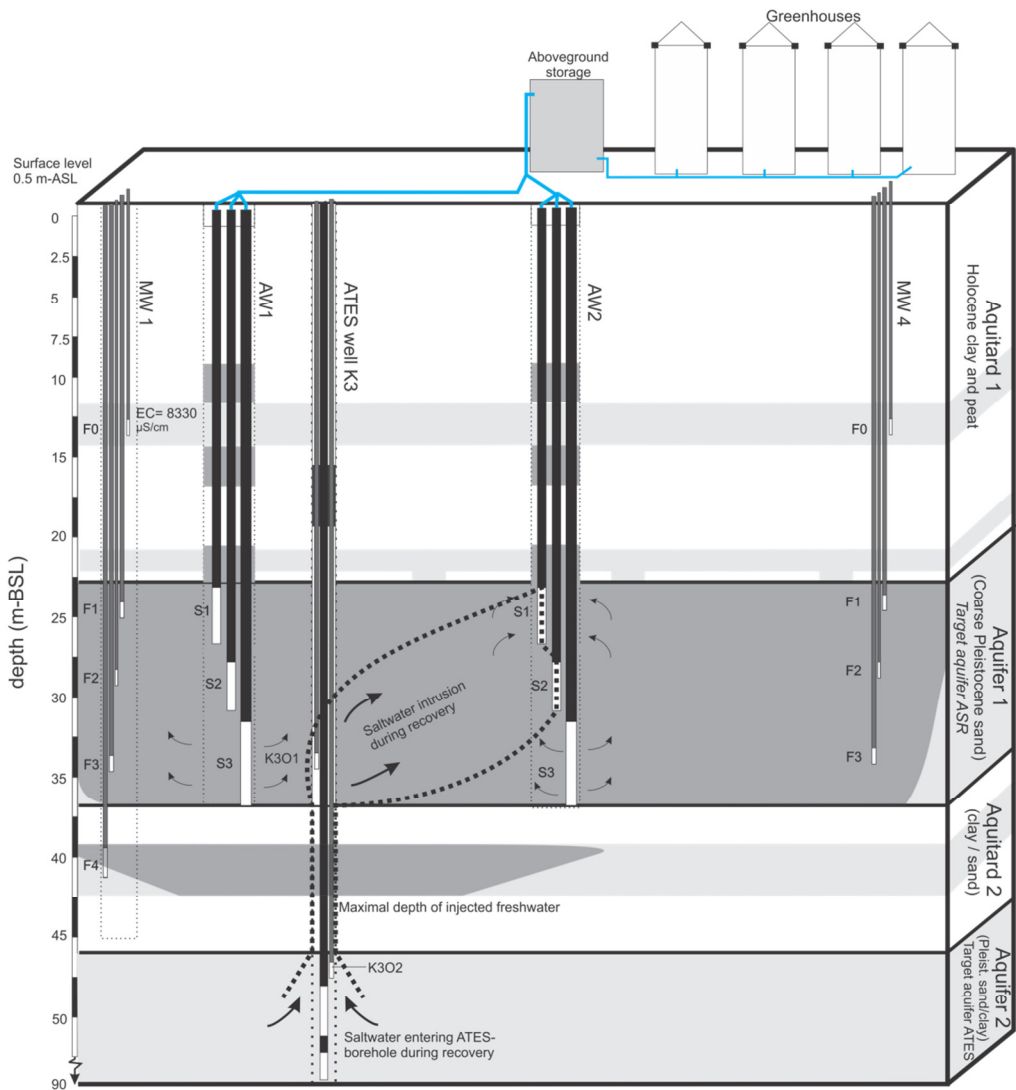
Figure 13: Deep saltwater intrusion via a borehole during recovery of injected freshwater at the Westland ASR site.
