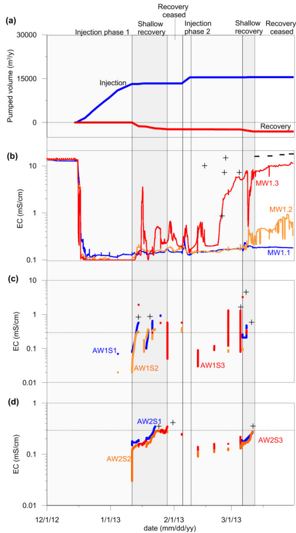
Figure 8: Pumping of the ASR system during cycle 1 in 2012/2013 (a), EC observations at MW1 at 5 m from AW1 (b), and the EC in the recovered water at AW1 (c) and AW2 (d).
