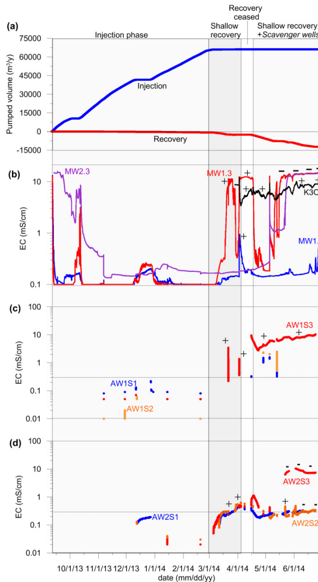
Figure 10: Pumping of the ASR system during Cycle 2 in 2013/2014 (a), EC observations at MW1 at 5 m from AW1 (b), and the EC in the recovered water at AW1 (c) and AW2 (d). AW2.1 and AW2.3 were used for freshwater recovery (12,324 m 3 ). Presence of increased \text{SO}_4 -concentrations (deep saltwater from Aquifer 2) are marked by '+', while its absence is marked by '-' (indicating shallow saltwater from Aquifer 1).
